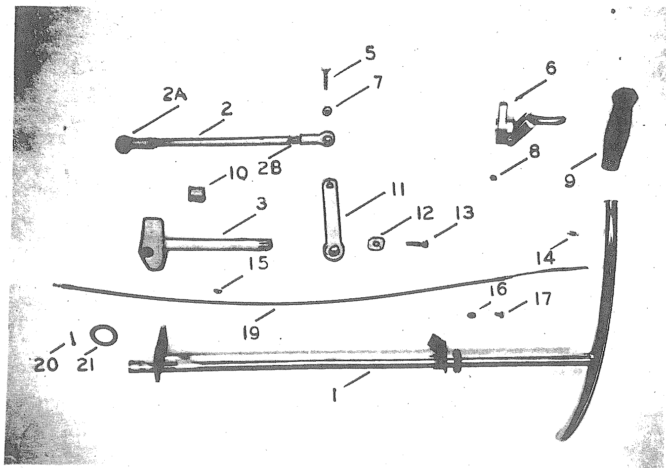
STEERING SECTION
